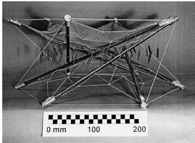
Fig. 17 Side view of model structure, expanded.
